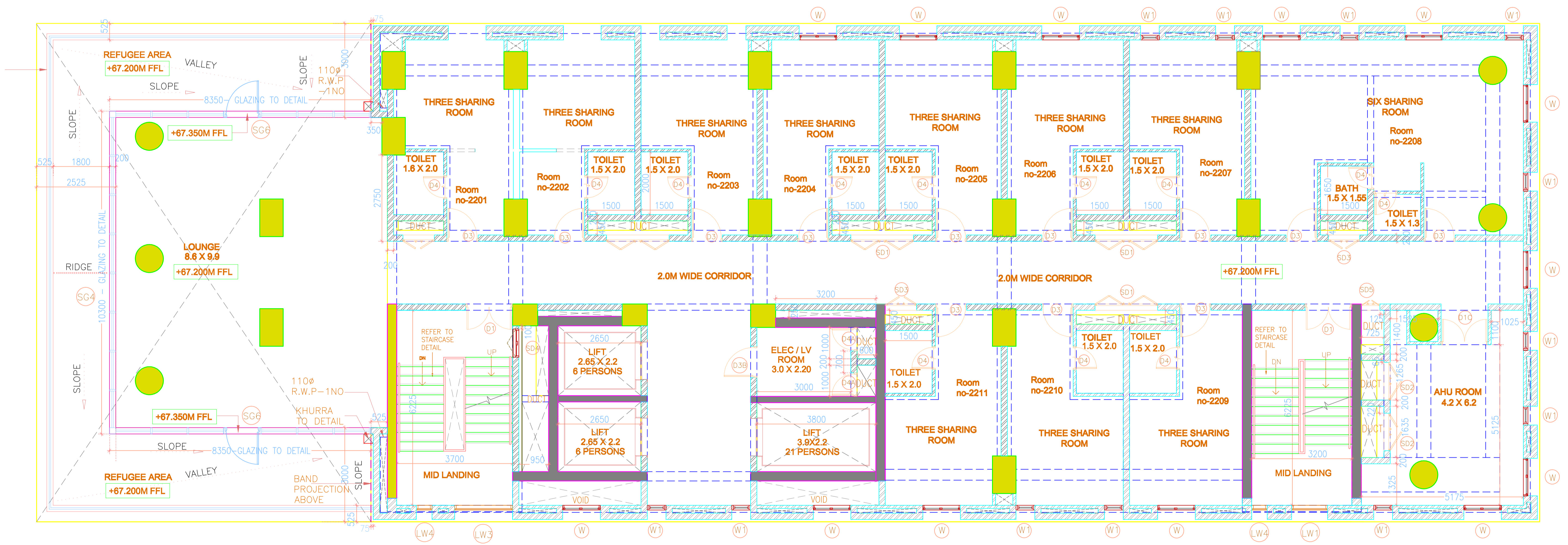
LEVEL - 22 FLOOR PLAN
