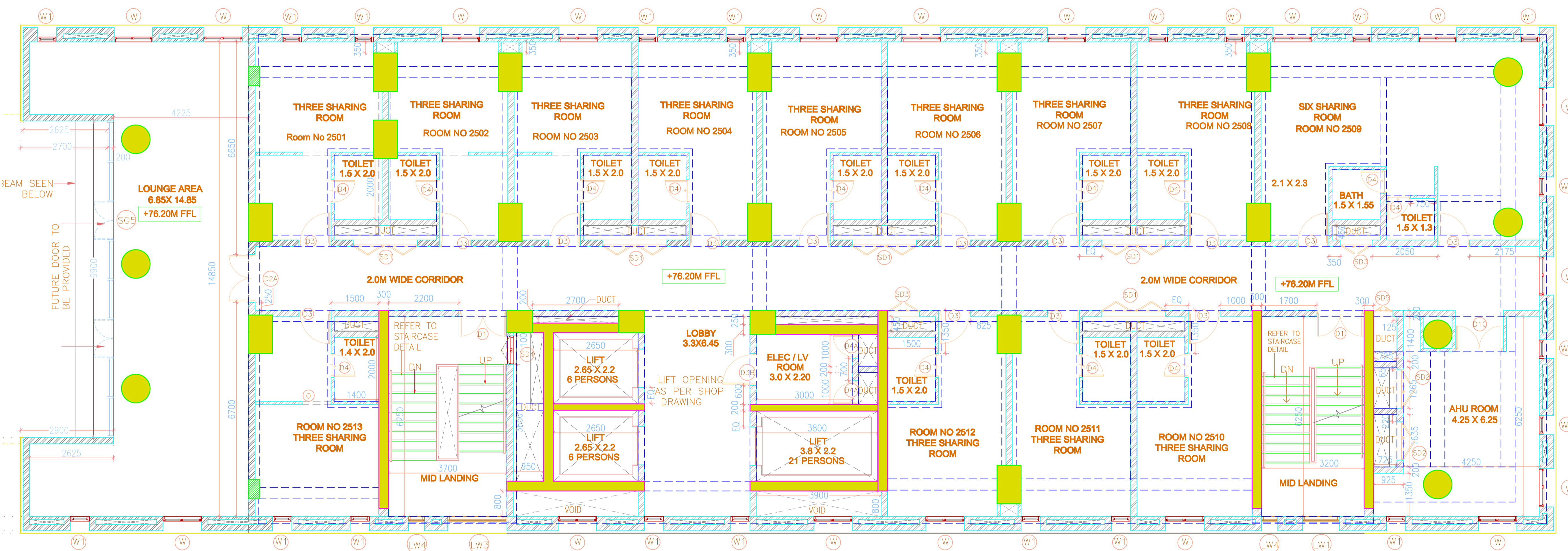
LEVEL - 25 (76.20M FFL) PLAN
